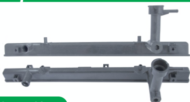
7916 / Jac 2 1.4/16V manual superior
